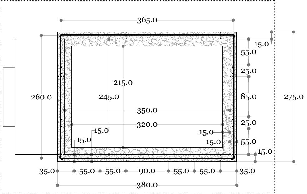
SECTIONS / FOUNDATION _I-A.03_
