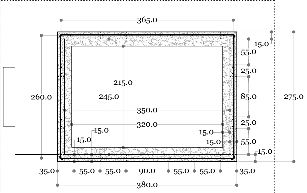
SECTIONS / FOUNDATION _I-A.03_
